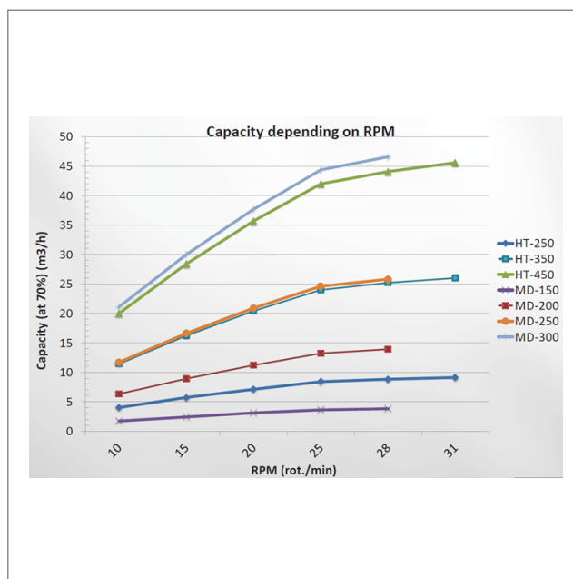
Capacity diagram for rotary valves HT/HT-S/MD
